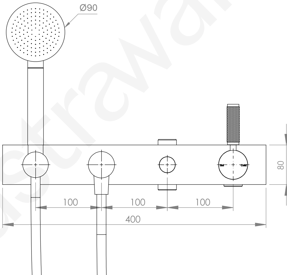
DIVERTER VIEW
