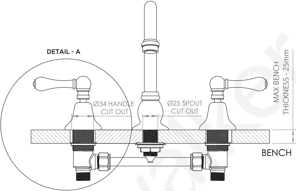
DETAIL - A CROSS SECTION
