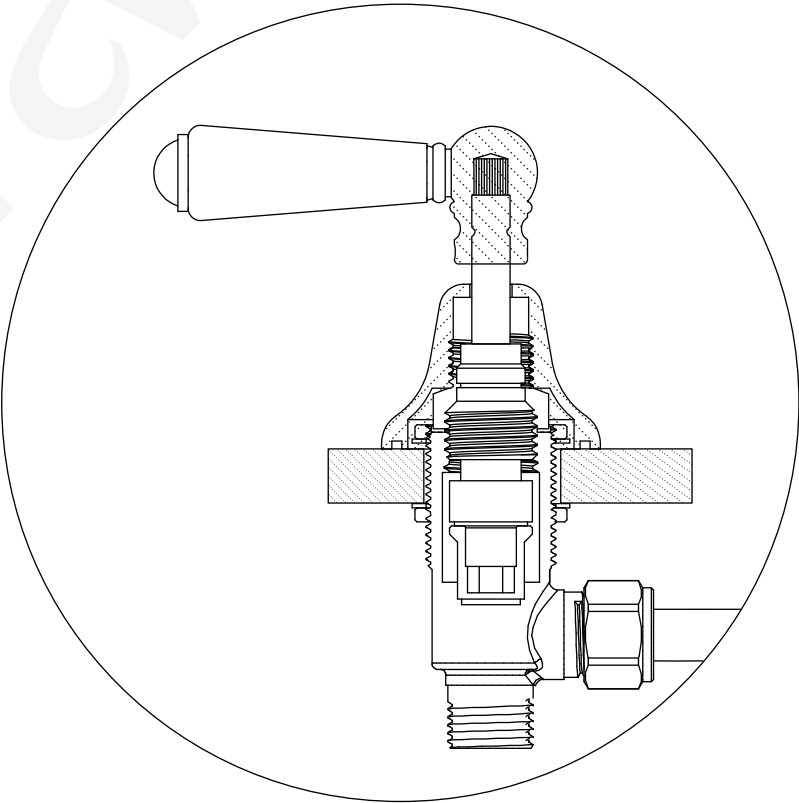
DETAIL - A CROSS SECTION
