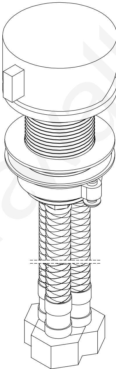
EXPLODED VIEW
