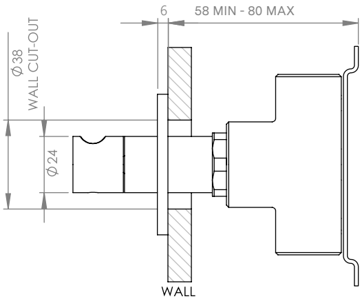
DIVERTER VIEW
