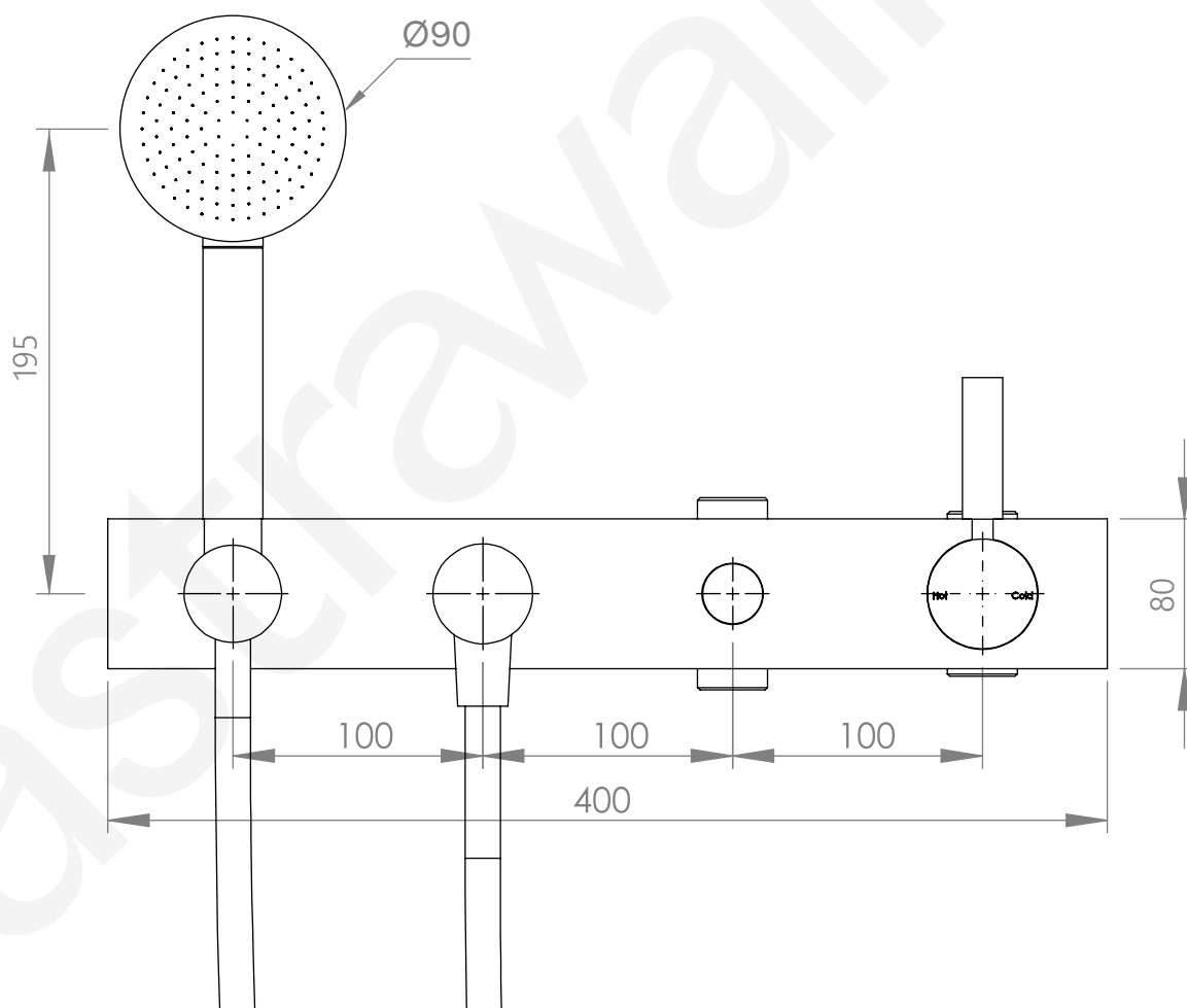
DIVERTER VIEW
