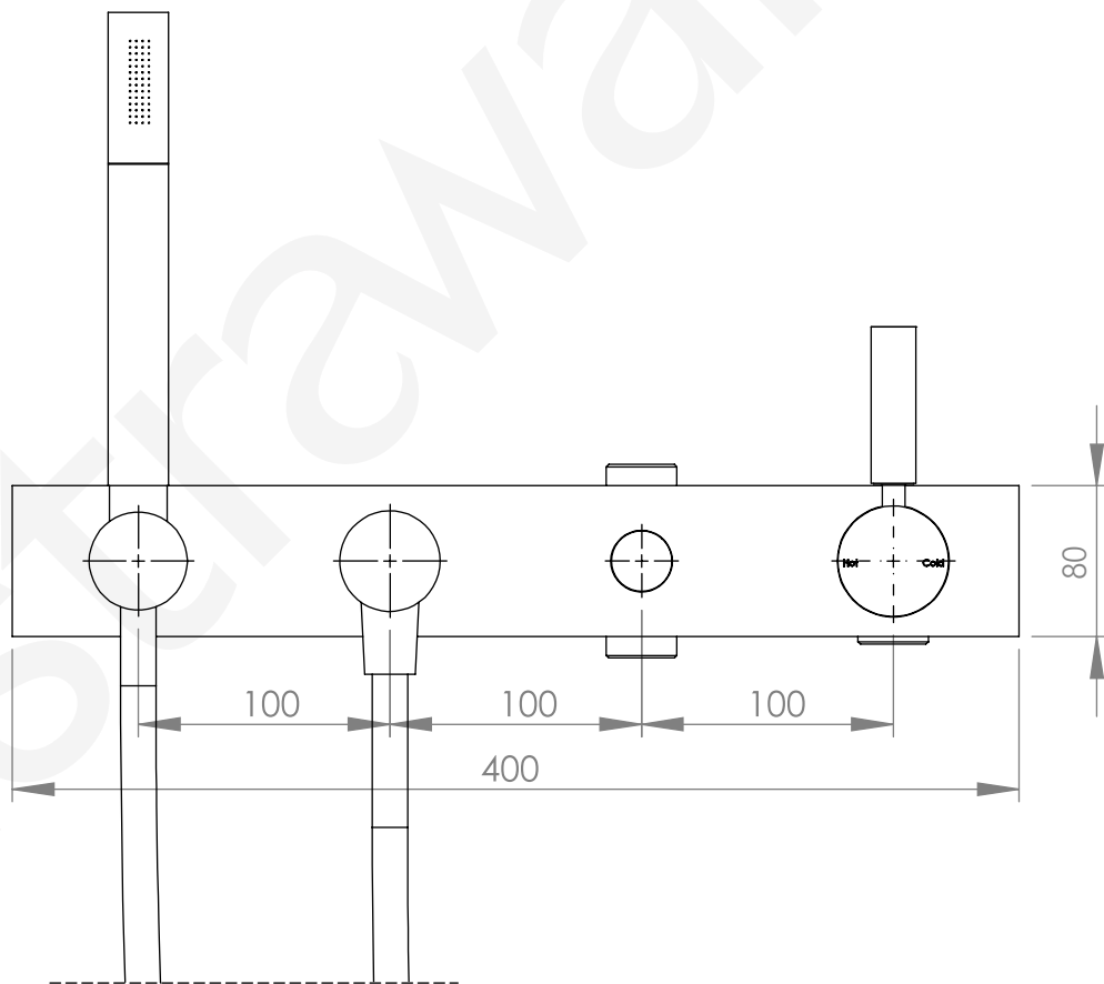
DIVERTER VIEW
