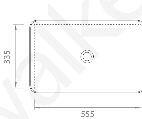
FURNITURE'S CUT OUT FOR BUILT-IN INSTALLATION
