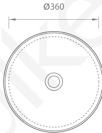
FURNITURE'S CUT OUT FOR BUILT-IN INSTALLATION
