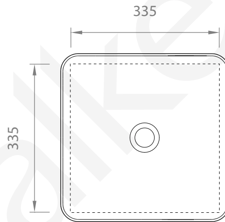
FURNITURE'S CUT OUT FOR BUILT-IN INSTALLATION
