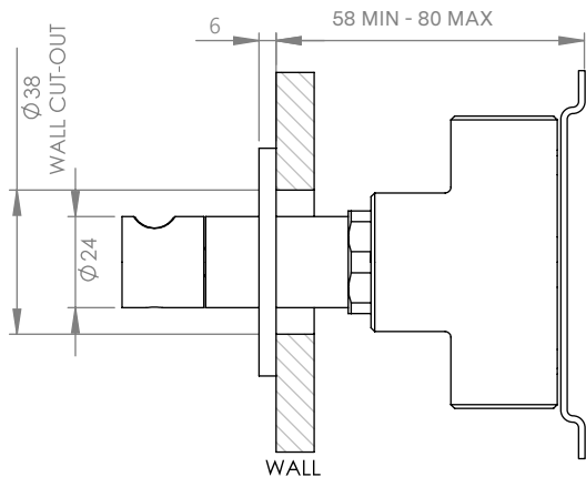
DIVERTER VIEW
