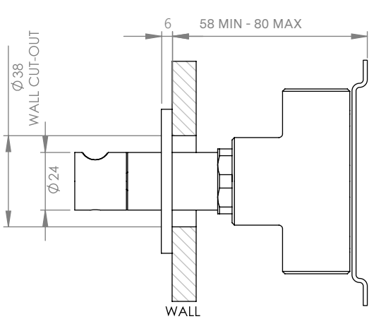
DIVERTER VIEW
